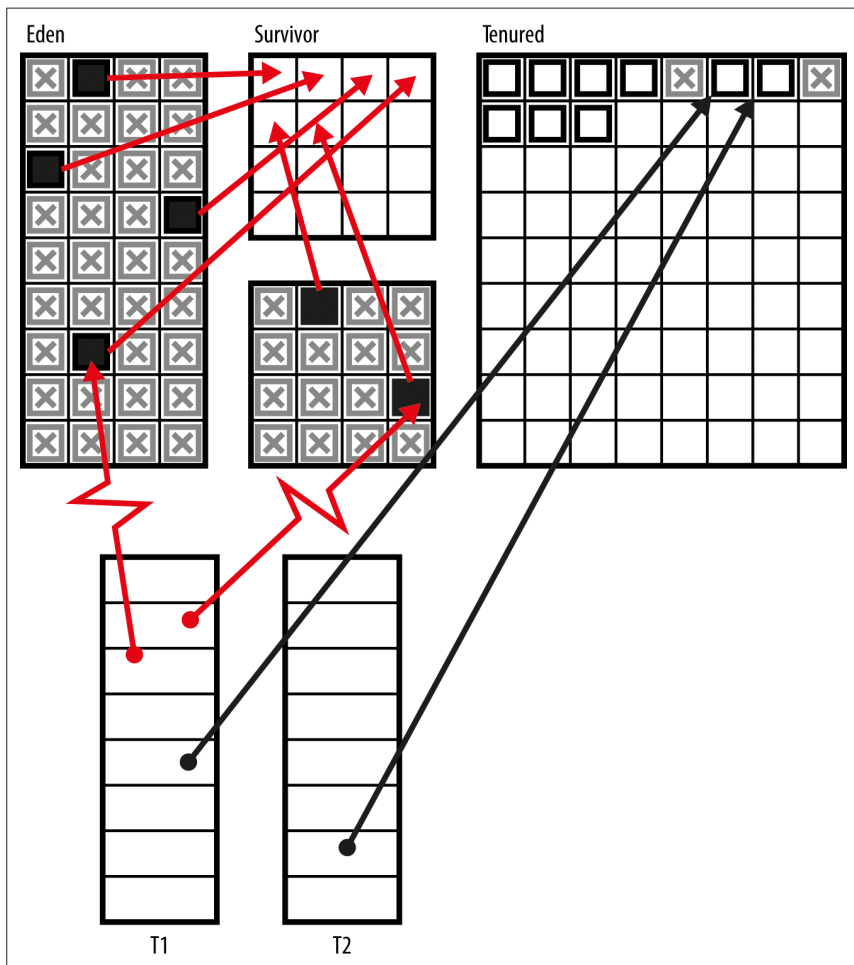
Figure 6-1. Heap mutation
