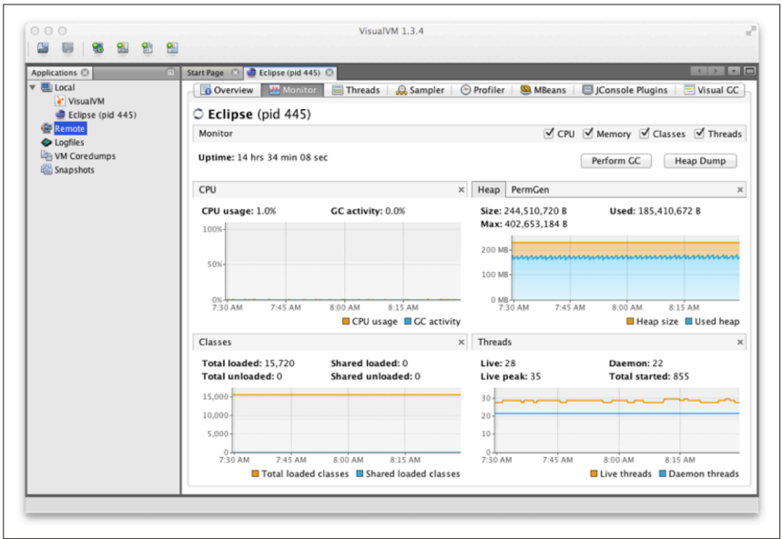
Figure 13-3. Monitor tab
